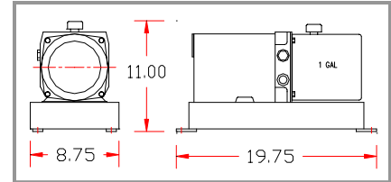
1 Hp Hydraulic Power Unit (Not in scale)
